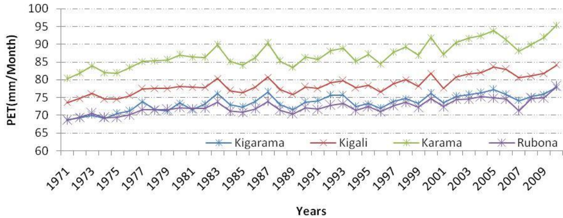
Figure 13. 30 years record for monthly average PET for Kigarama, Karama, Rubona and Kigali station for 1971-2010.
