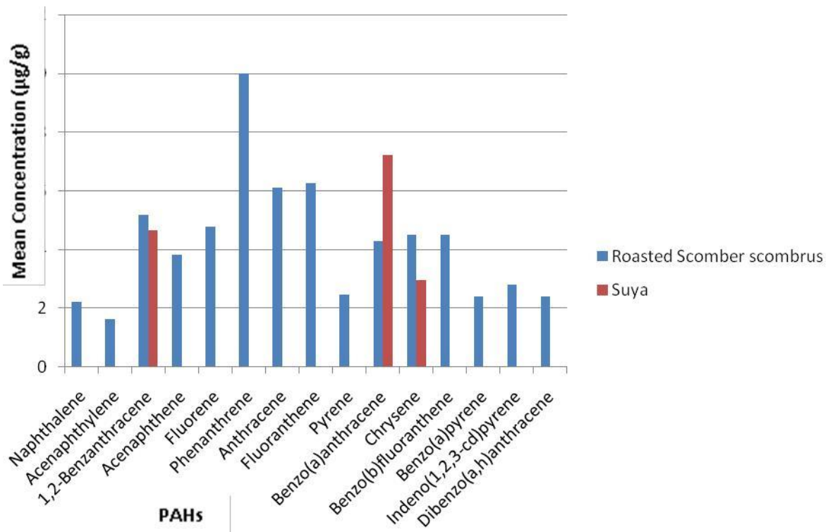
Figure 2. PAH Distribution in Roasted Scomber scombrus and Suya beef.
