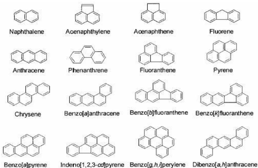
Figure 1. Chemical Structure of Some PAHs.
